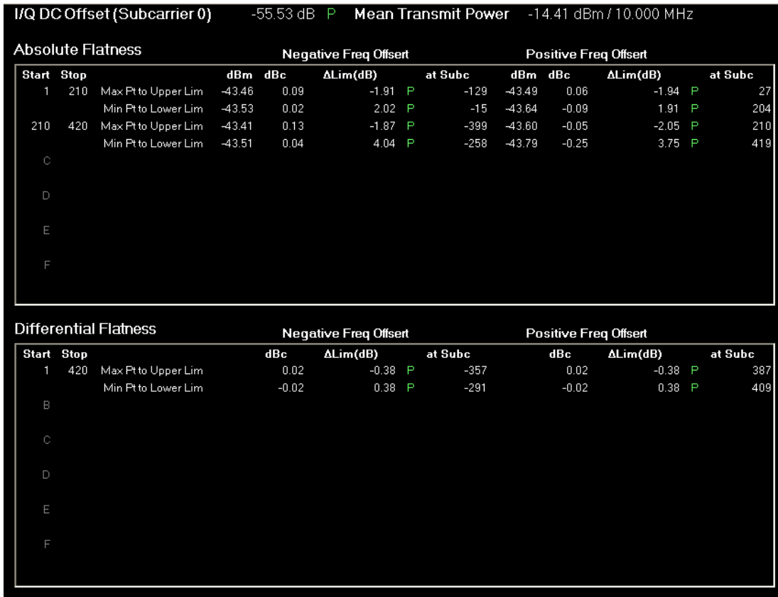
Figure 1 Zoomed Spectral Flatness Result Metrics Window
